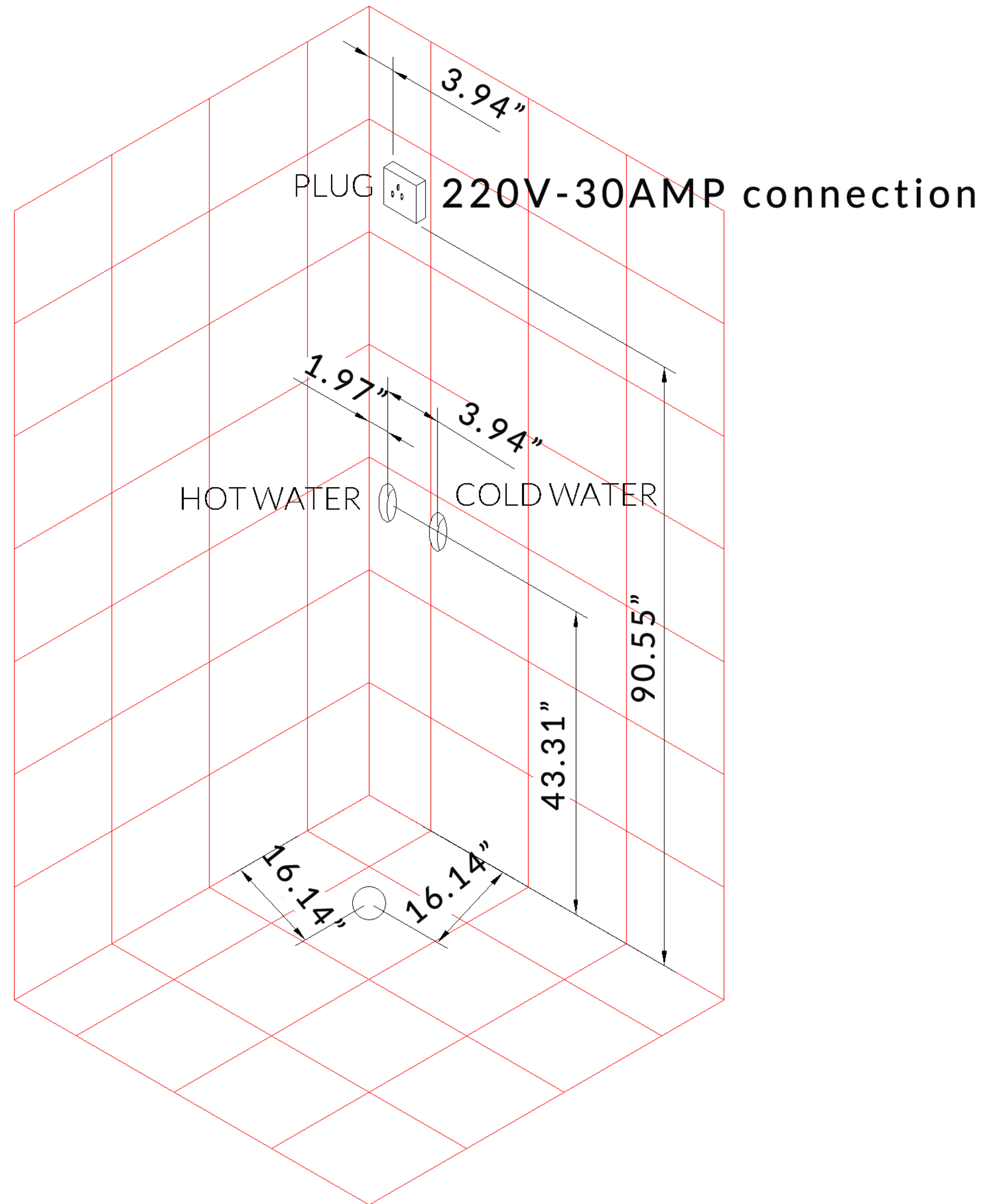
DZ959F8 INSTALLATION(RIGHT) DIMENSIONS: 47" x 35" x 89"
